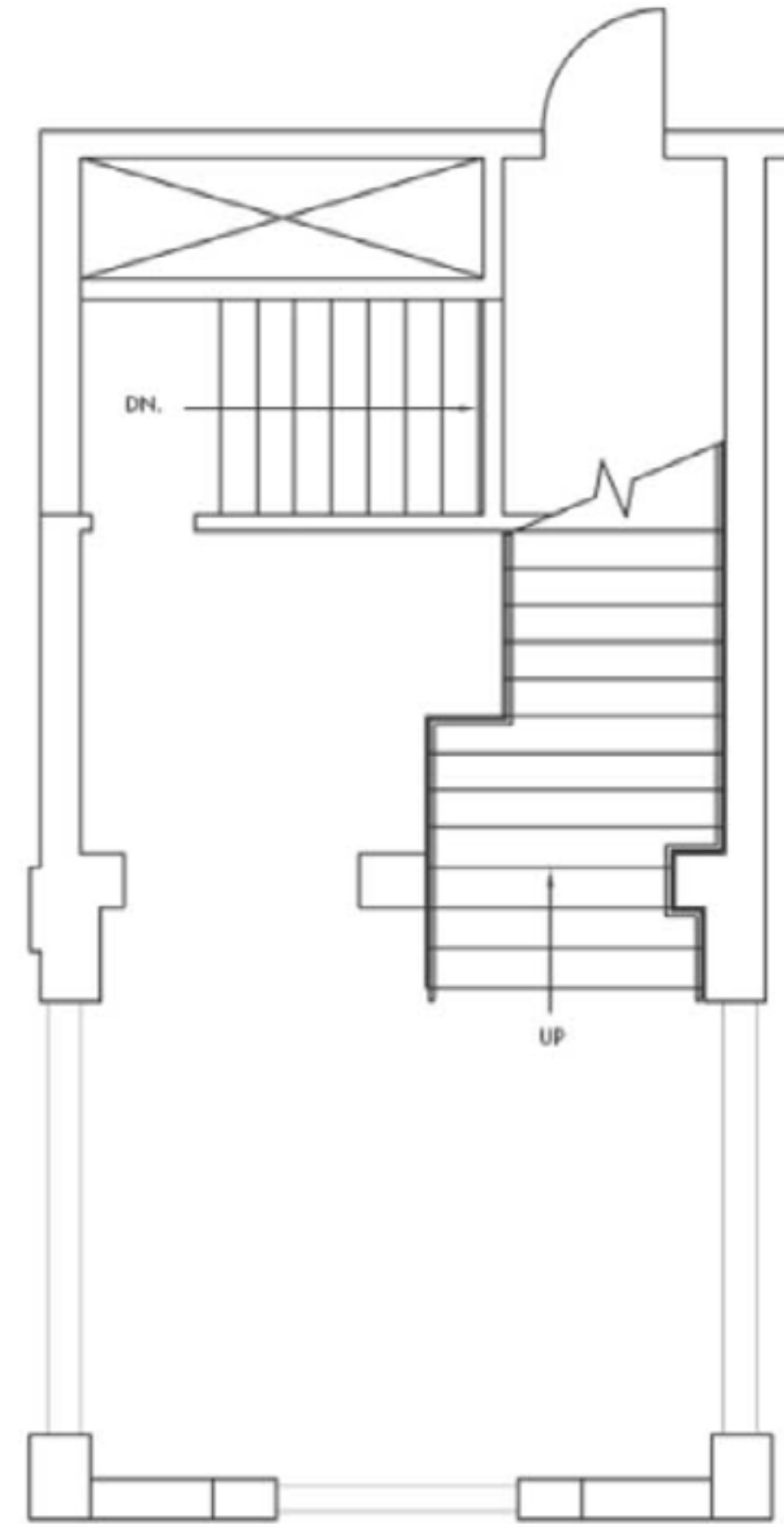
THE VESTIBULE FLOOR PLAN
